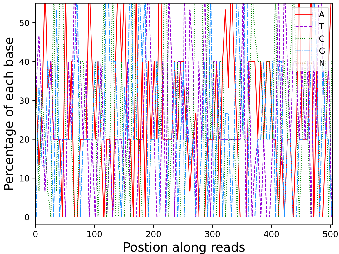
Base percentage along reads (R10521)
